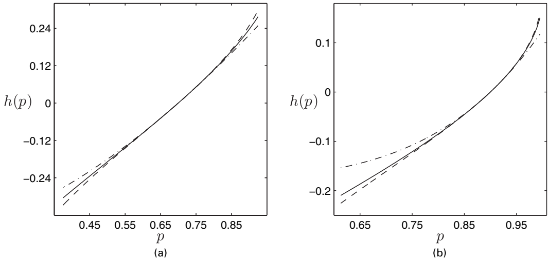
Fig. 3. Variance stabilizing transformations h(\rho) for the binomial parameter \rho (—, exact variance stabilizing transformation; - - -, Box-Cox transformation applied to odds \omega = \rho/(1 - \rho) ; · - · - ·, Box-Cox transformation applied to \rho ): (a) \hat{\rho} = 0.7 ; (b) \hat{\rho} = 0.9
