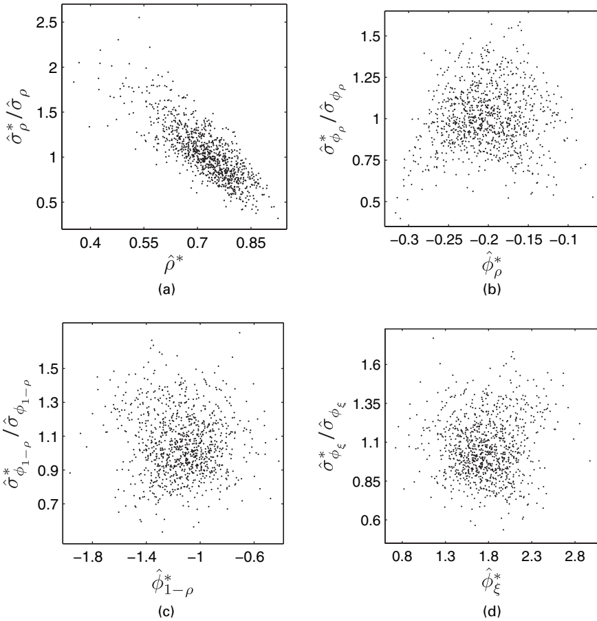
Fig. 2. Standard deviation versus parameter plots for correlation coefficient \rho ( B = 999 ): (a) \rho ; (b) \hat{\phi}_\rho , the Box–Cox transformation applied to \rho ; (c) \hat{\phi}_{1-\rho} , the Box–Cox transformation applied to 1 - \rho ; (d) \hat{\phi}_\xi , the Box–Cox transformation applied to \xi = (1 + \rho)/(1 - \rho)
